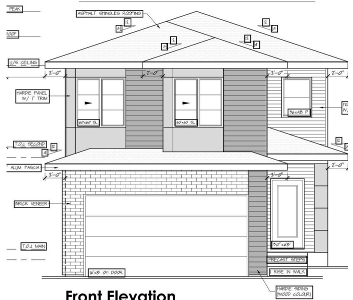
Front Elevation
